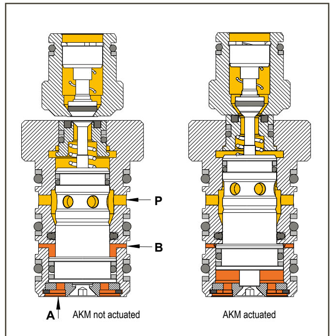
Functional schematic of the automatic coupling mechanism (AKM)
